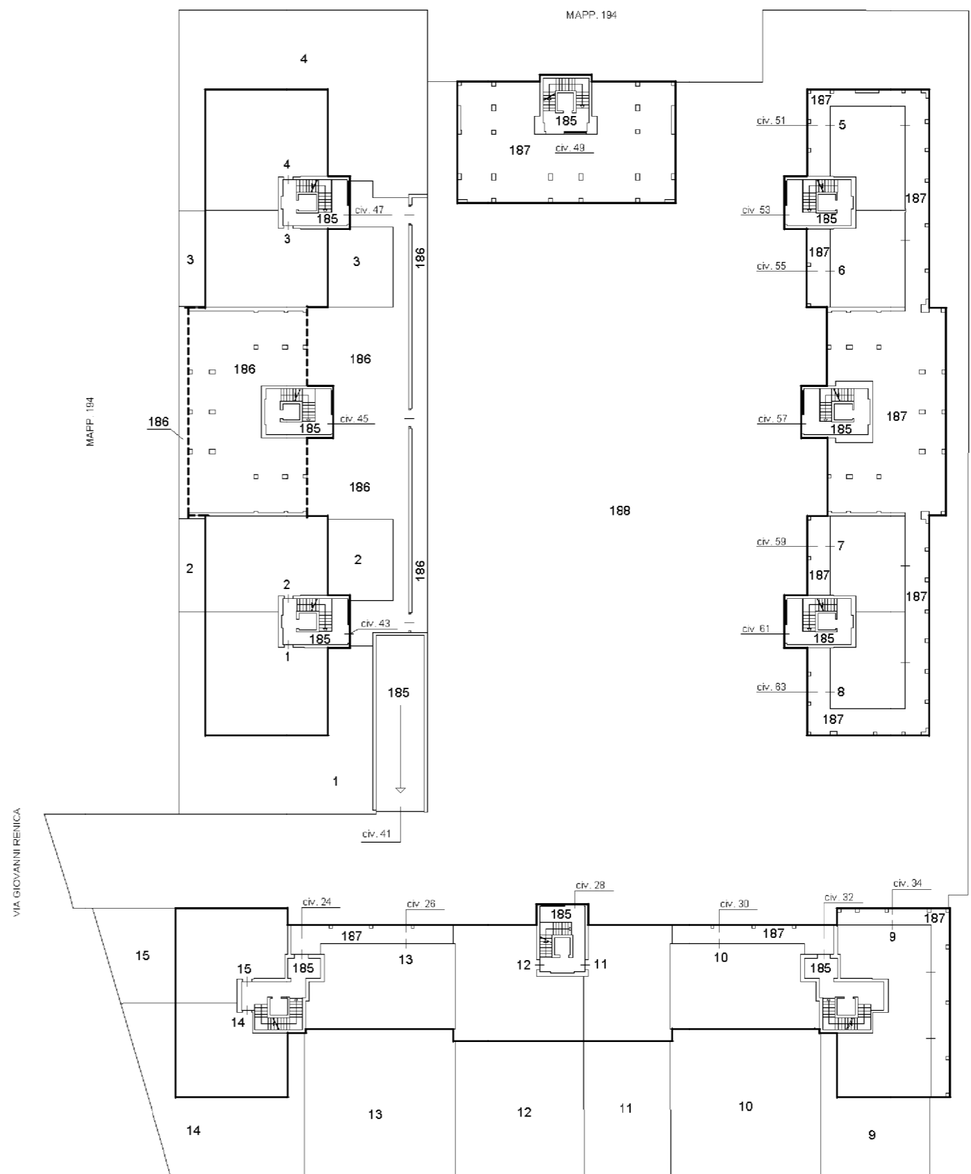
PIANO TERRA
